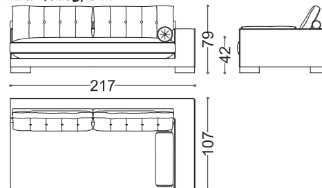
Art. 40205/SX
