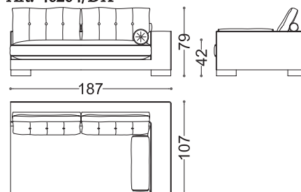
Art. 40204/SX
