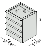
Cassettiera 4 cassetti 63 4 Drawers chest 63
