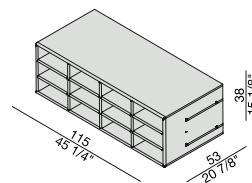
Alveare 120 Pigeon hole 120
