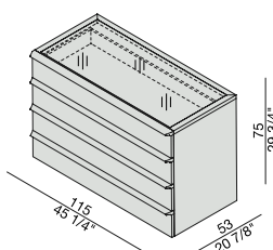
Cassettiera 4 cassetti 120 4 Drawers chest 120
