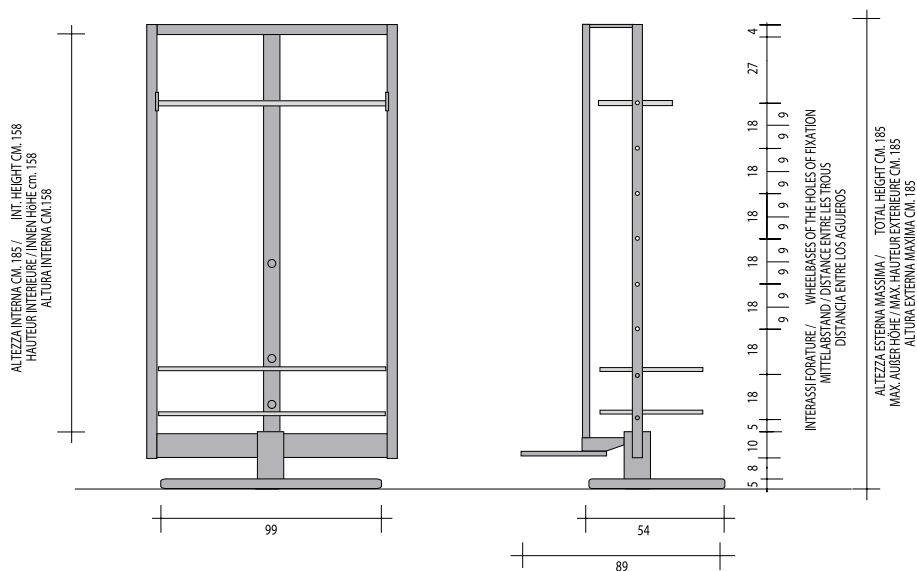
COMP. U42
