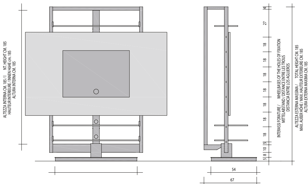
COMP. U47
