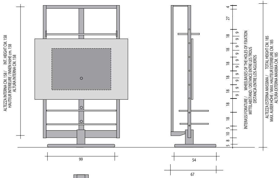
COMP. U41
