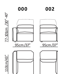
chair with arm
