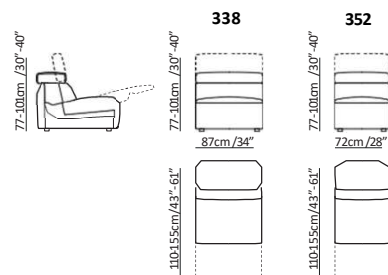
dual power motion armless chair
