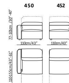
dual power motion chair with arm
