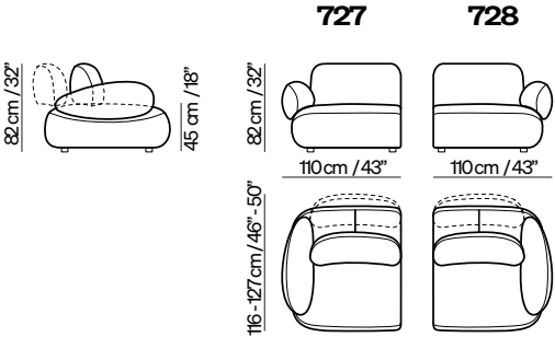
Power sliding backrest chair with arm
