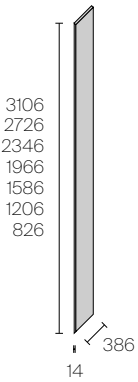
Aluminium side panel
